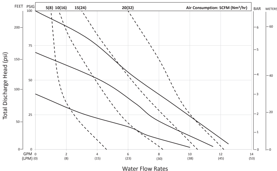
PF66605 Performance
